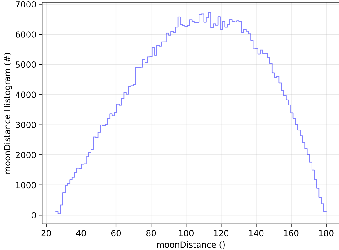
early_ss_template_fpextra2.0_v3.4_10yrs All sky r band: moonDistance Histogram
