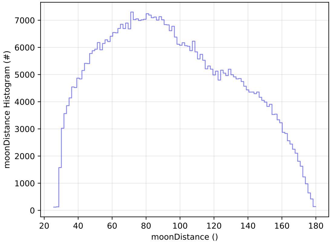
early_ss_template_fpextra2.0_v3.4_10yrs All sky i band: moonDistance Histogram
