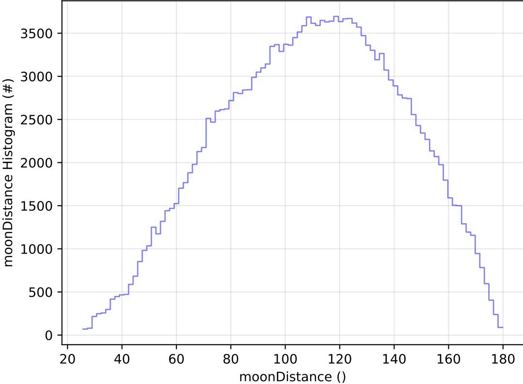
early_ss_template_fpextra2.0_v3.4_10yrs All sky g band: moonDistance Histogram
