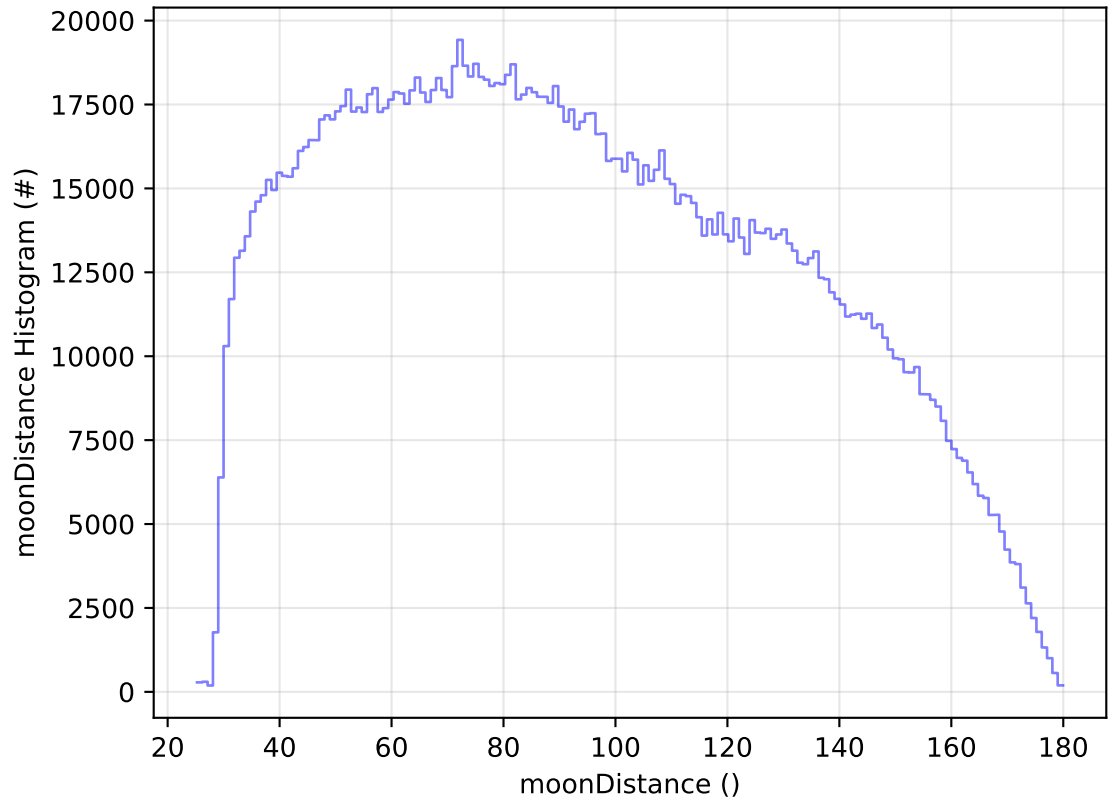
early_ss_template_fpextra2.0_v3.4_10yrs All sky all bands: moonDistance Histogram
