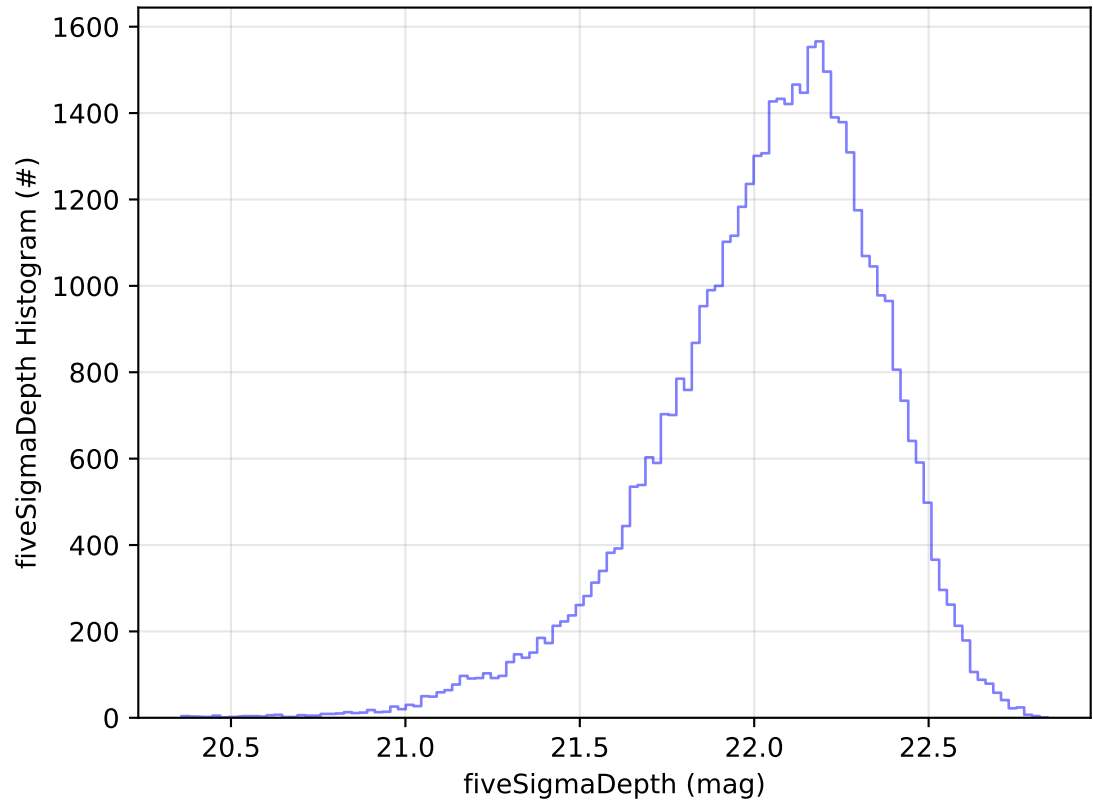
early_ss_template_fpextra2.0_v3.4_10yrs Yr 1 y band: fiveSigmaDepth Histogram
