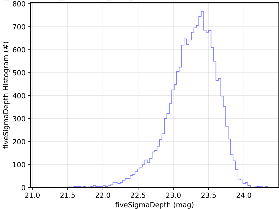
early_ss_template_fpextra2.0_v3.4_10yrs Yr 1 u band: fiveSigmaDepth Histogram
