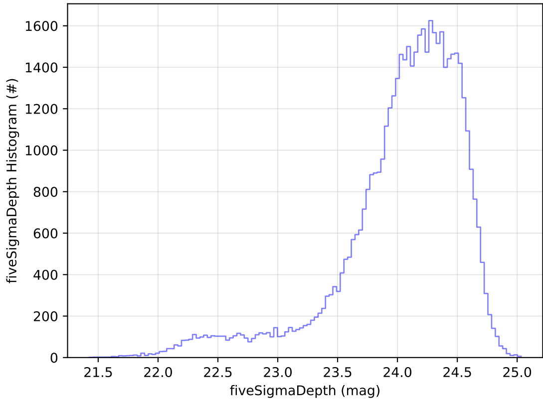
early_ss_template_fpextra2.0_v3.4_10yrs Yr 1 r band: fiveSigmaDepth Histogram
