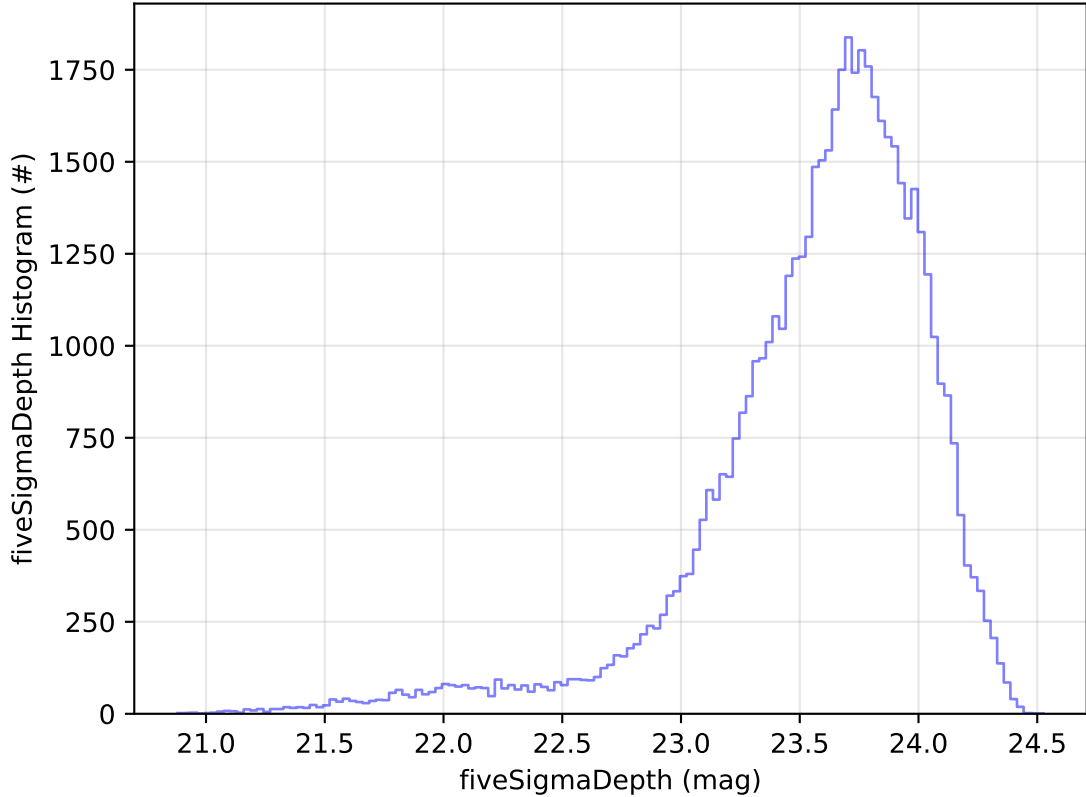
early_ss_template_fpextra2.0_v3.4_10yrs Yr 1 i band: fiveSigmaDepth Histogram
