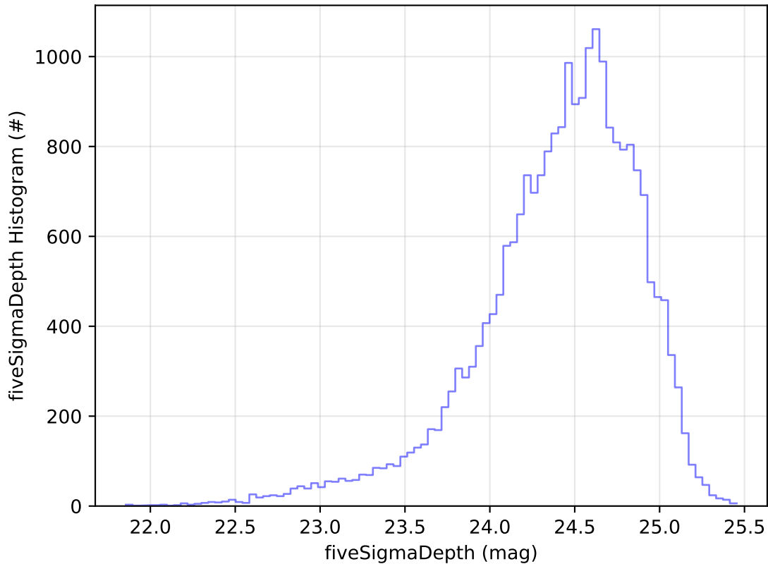
early_ss_template_fpextra2.0_v3.4_10yrs Yr 1 g band: fiveSigmaDepth Histogram
