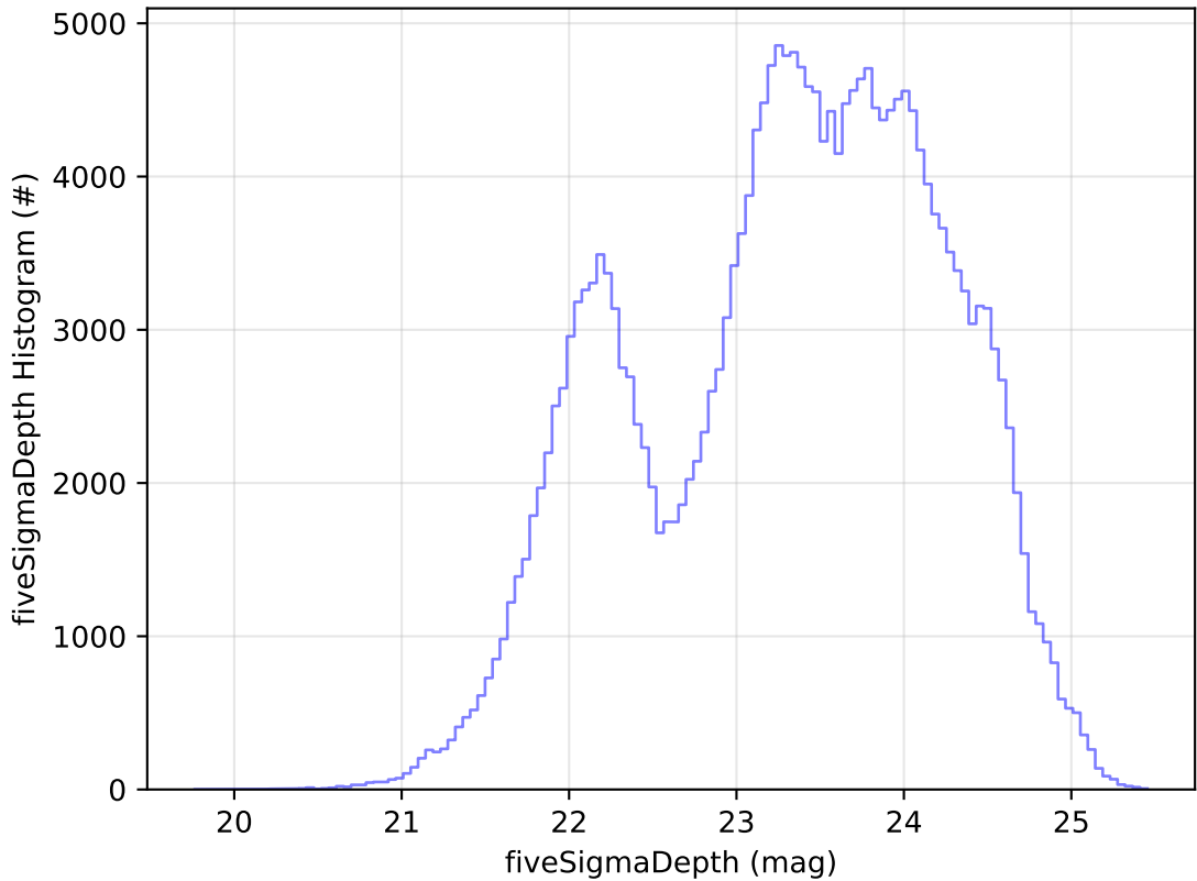
early_ss_template_fpextra2.0_v3.4_10yrs Yr 1 all bands: fiveSigmaDepth Histogram
