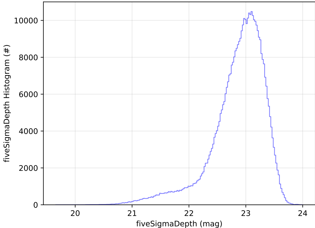
early_ss_template_fpextra2.0_v3.4_10yrs WFD z band: fiveSigmaDepth Histogram
