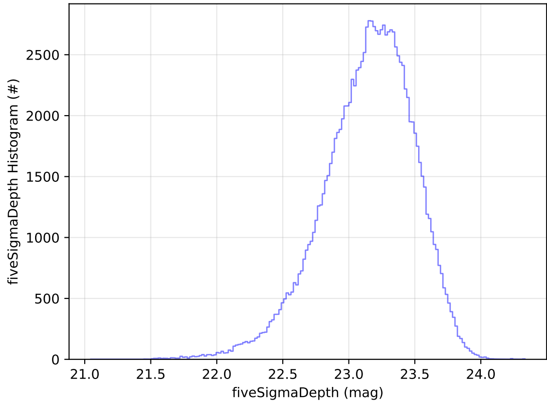
early_ss_template_fpextra2.0_v3.4_10yrs WFD u band: fiveSigmaDepth Histogram
