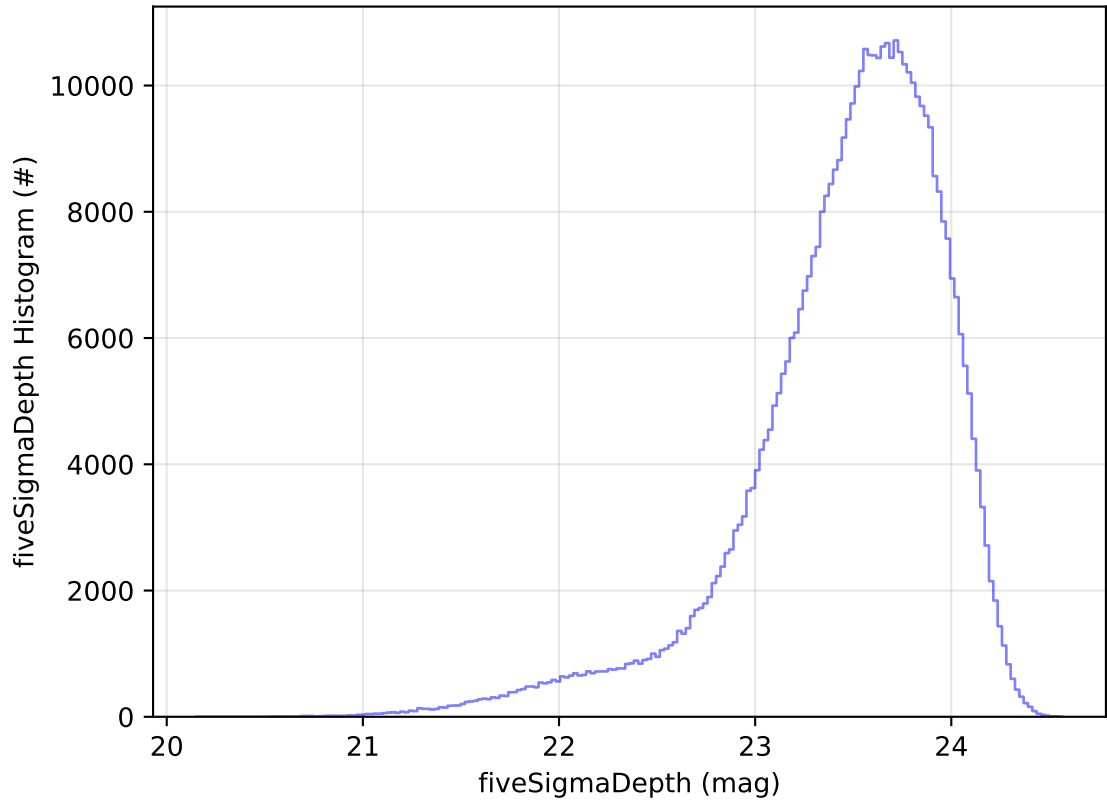
early_ss_template_fpextra2.0_v3.4_10yrs WFD i band: fiveSigmaDepth Histogram
