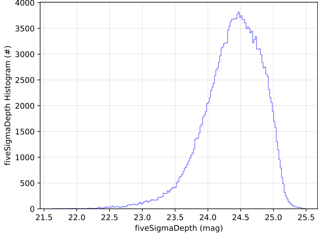
early_ss_template_fpextra2.0_v3.4_10yrs WFD g band: fiveSigmaDepth Histogram
