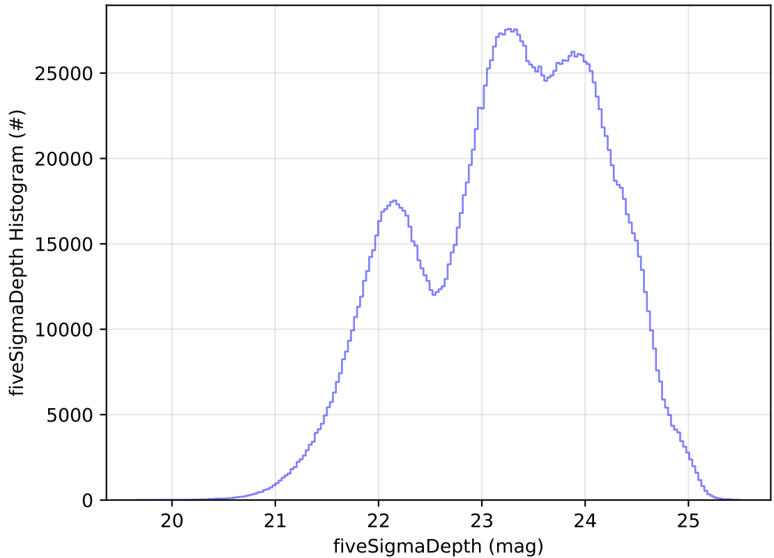
early_ss_template_fpextra2.0_v3.4_10yrs WFD all bands: fiveSigmaDepth Histogram
