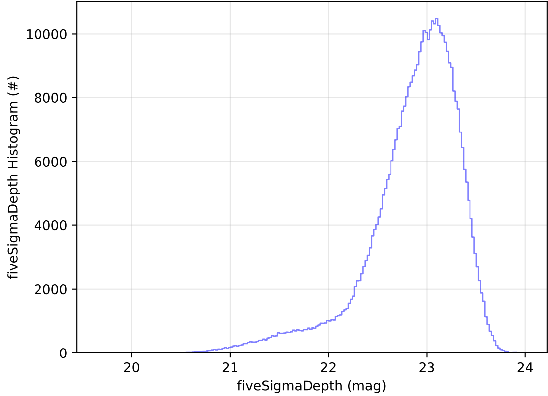
early_ss_template_fpextra2.0_v3.4_10yrs All sky z band: fiveSigmaDepth Histogram
