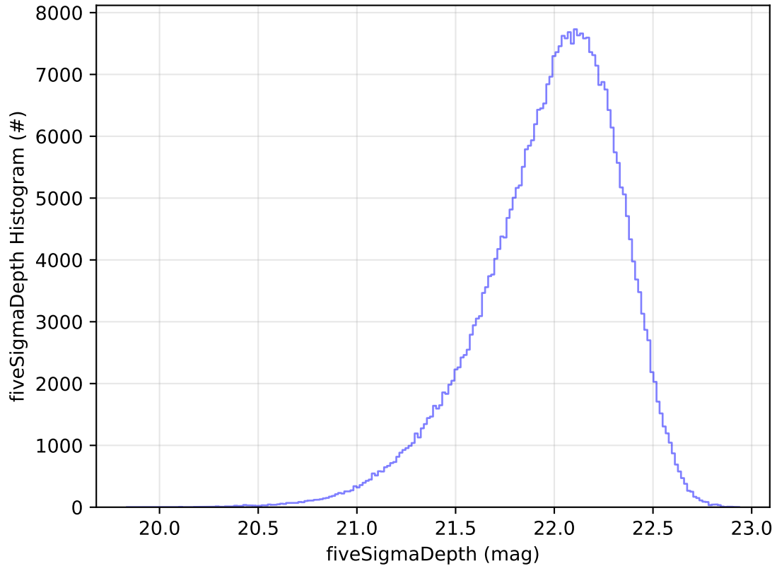
early_ss_template_fpextra2.0_v3.4_10yrs All sky y band: fiveSigmaDepth Histogram
