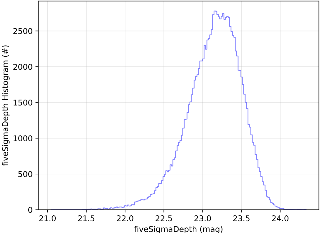
early_ss_template_fpextra2.0_v3.4_10yrs All sky u band: fiveSigmaDepth Histogram
