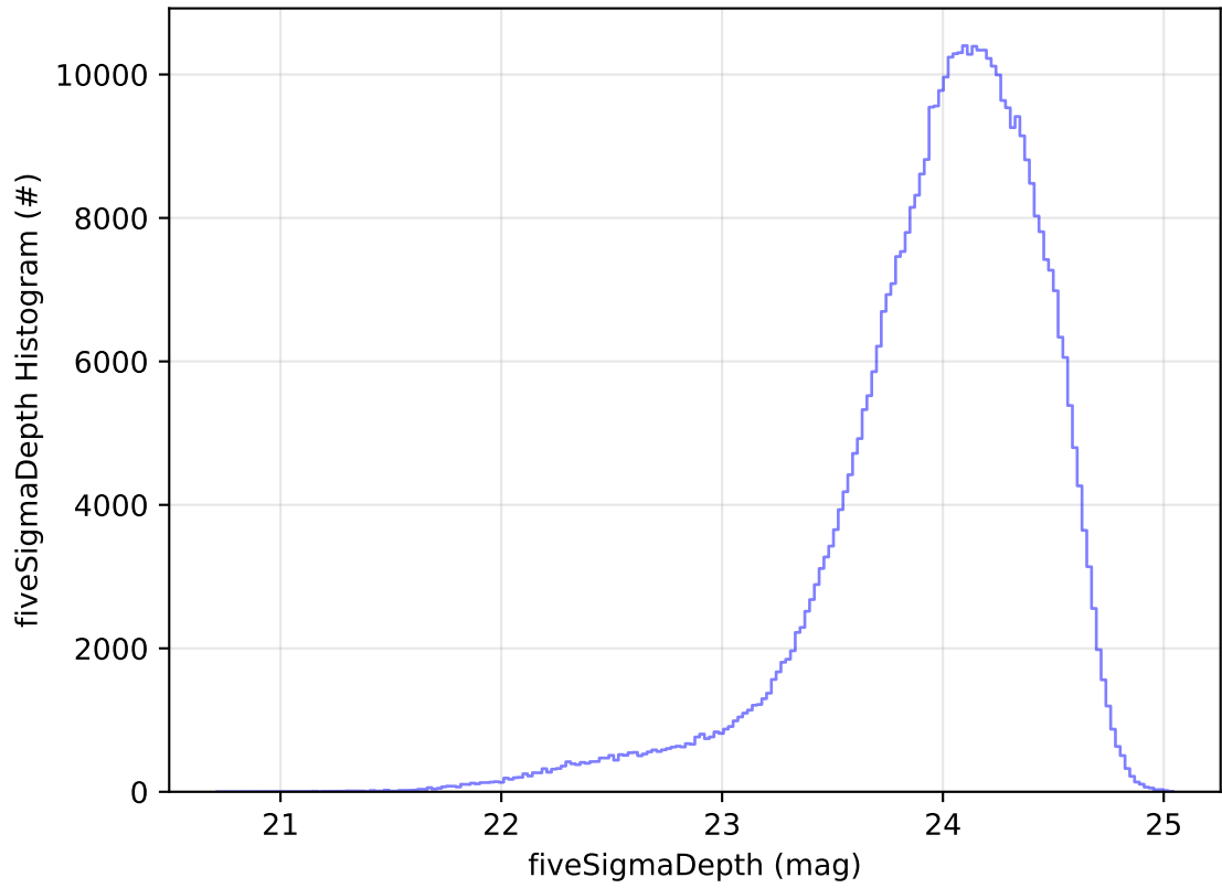
early_ss_template_fpextra2.0_v3.4_10yrs All sky r band: fiveSigmaDepth Histogram
