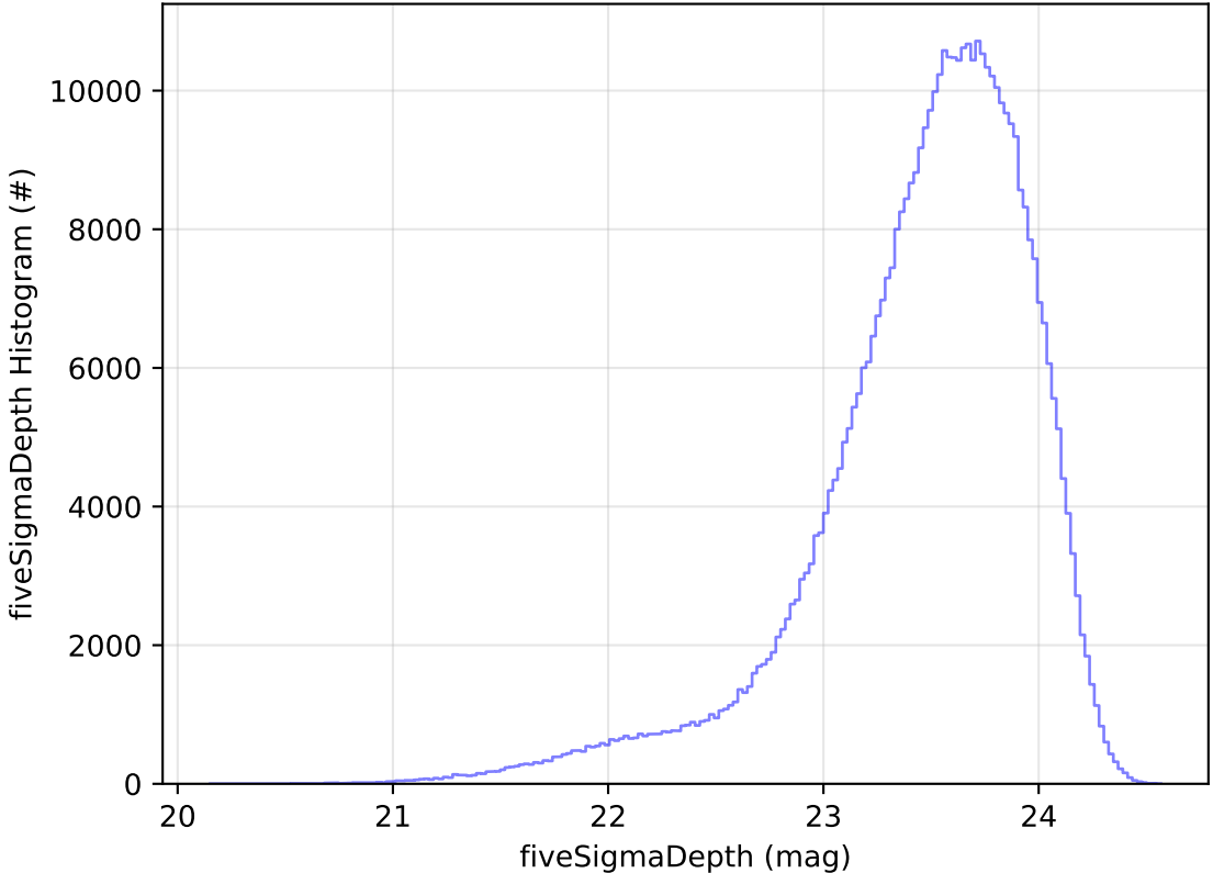
early_ss_template_fpextra2.0_v3.4_10yrs All sky i band: fiveSigmaDepth Histogram
