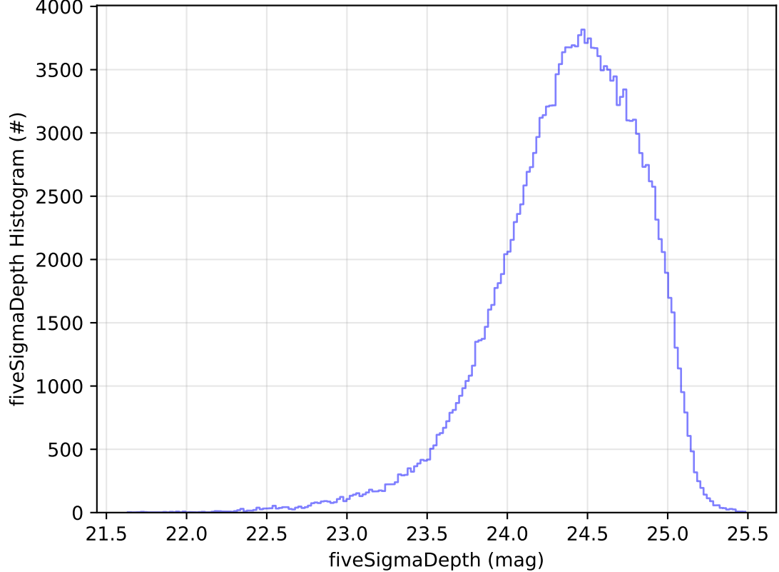
early_ss_template_fpextra2.0_v3.4_10yrs All sky g band: fiveSigmaDepth Histogram
