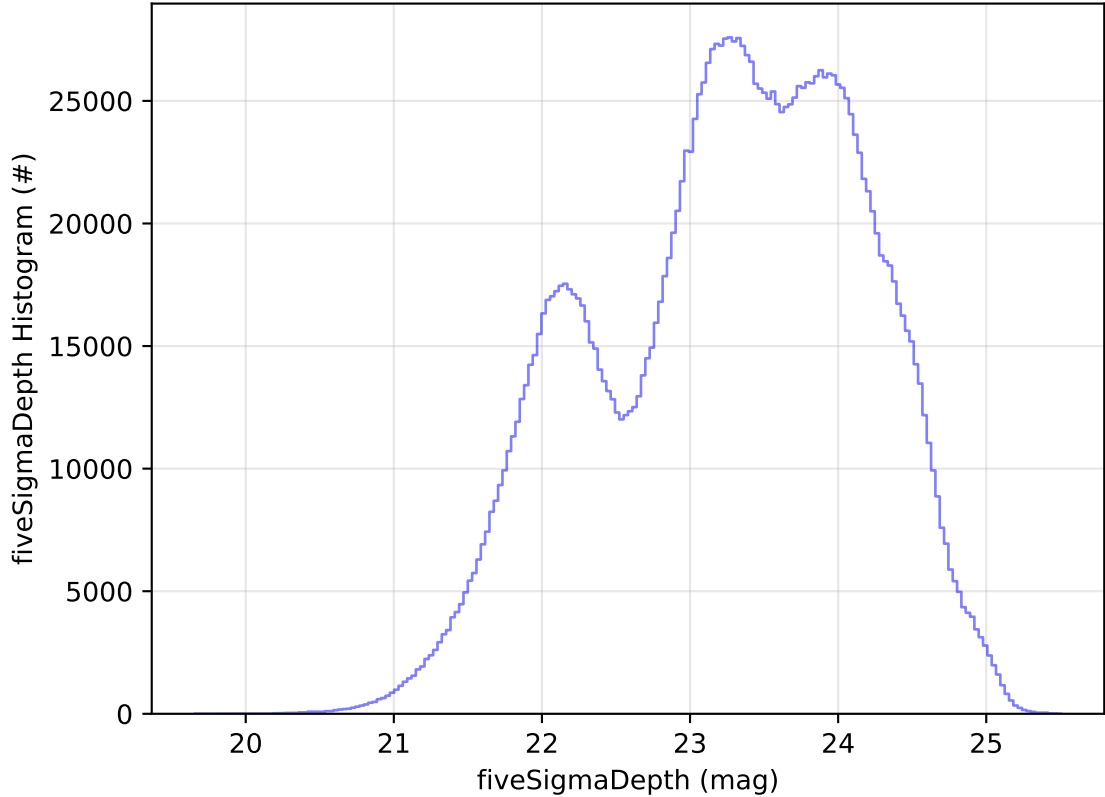
early_ss_template_fpextra2.0_v3.4_10yrs All sky all bands: fiveSigmaDepth Histogram
