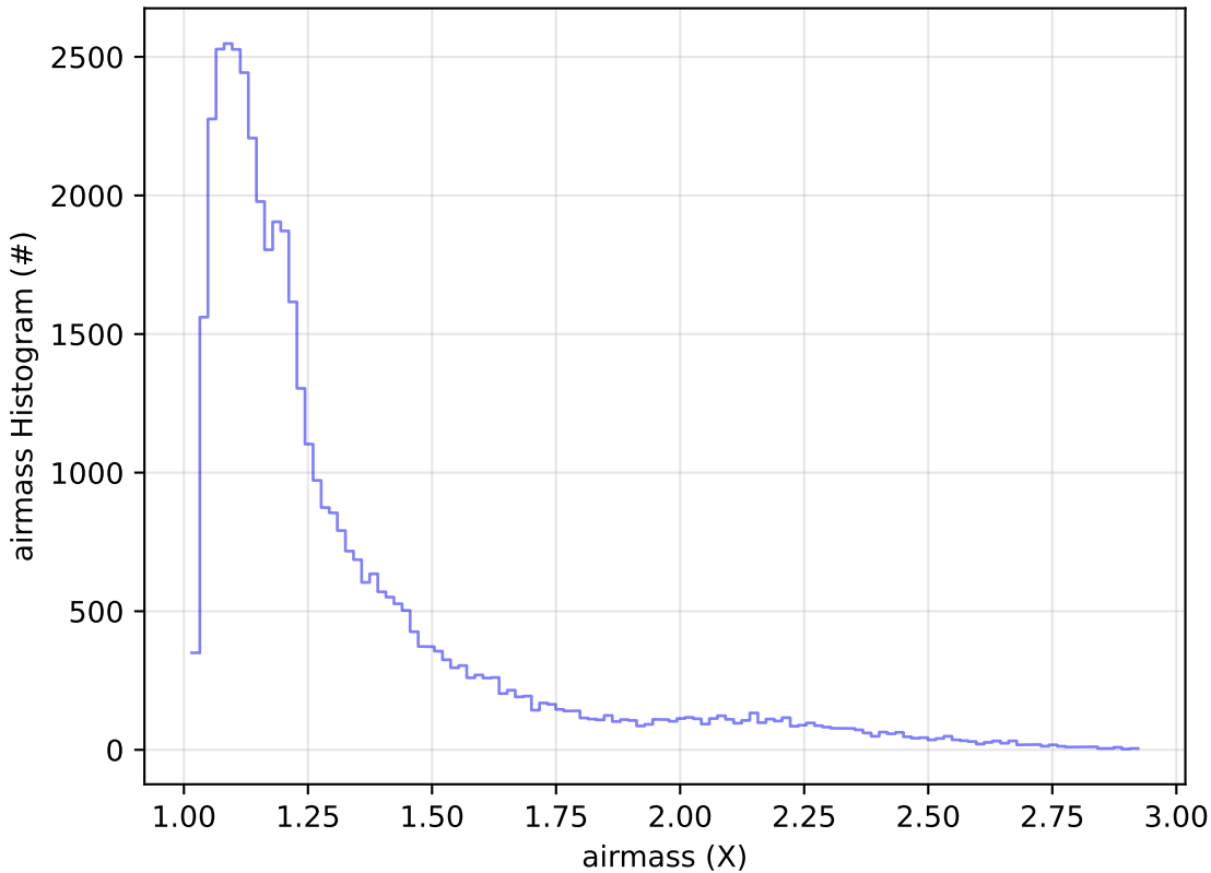
early_ss_template_fpextra2.0_v3.4_10yrs Yr 1 z band: airmass Histogram
