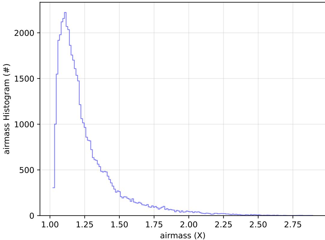
early_ss_template_fpextra2.0_v3.4_10yrs Yr 1 y band: airmass Histogram
