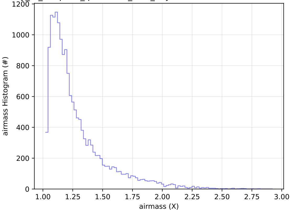
early_ss_template_fpextra2.0_v3.4_10yrs Yr 1 u band: airmass Histogram
