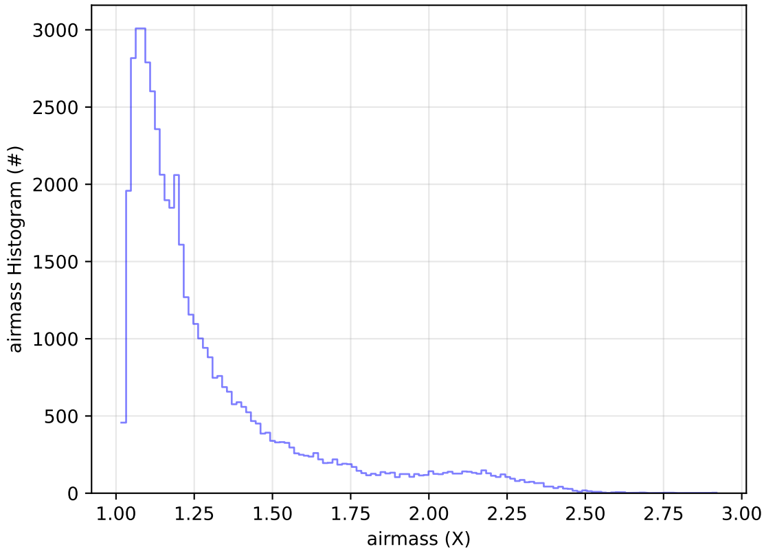
early_ss_template_fpextra2.0_v3.4_10yrs Yr 1 r band: airmass Histogram
