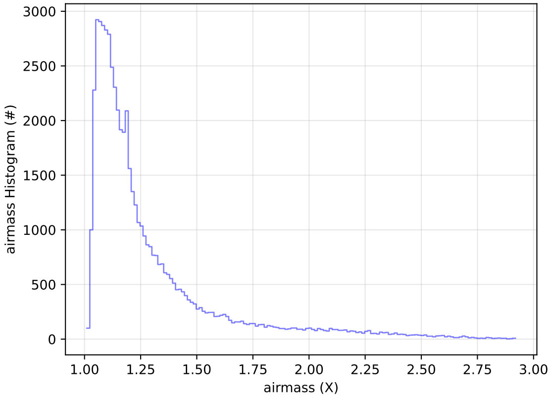
early_ss_template_fpextra2.0_v3.4_10yrs Yr 1 i band: airmass Histogram
