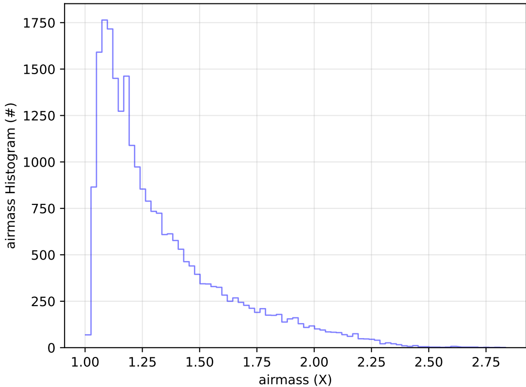
early_ss_template_fpextra2.0_v3.4_10yrs Yr 1 g band: airmass Histogram
