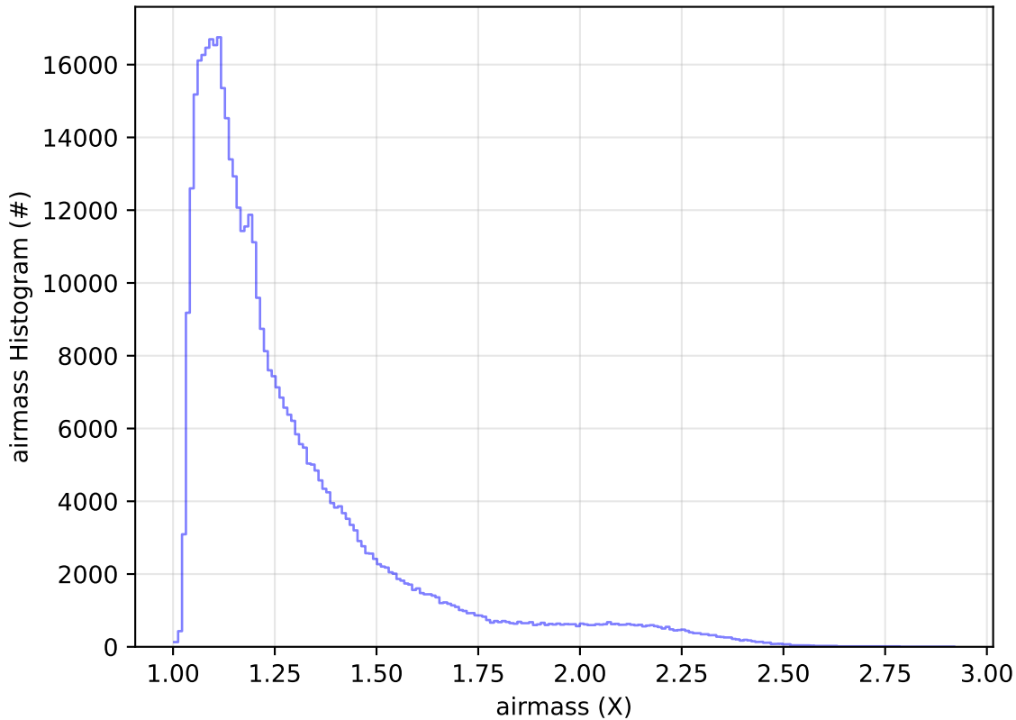
early_ss_template_fpextra2.0_v3.4_10yrs WFD r band: airmass Histogram
