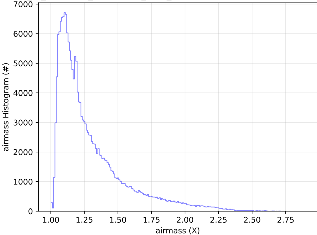
early_ss_template_fpextra2.0_v3.4_10yrs WFD g band: airmass Histogram
