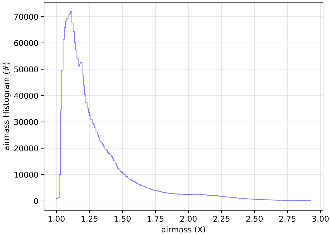
early_ss_template_fpextra2.0_v3.4_10yrs WFD all bands: airmass Histogram
