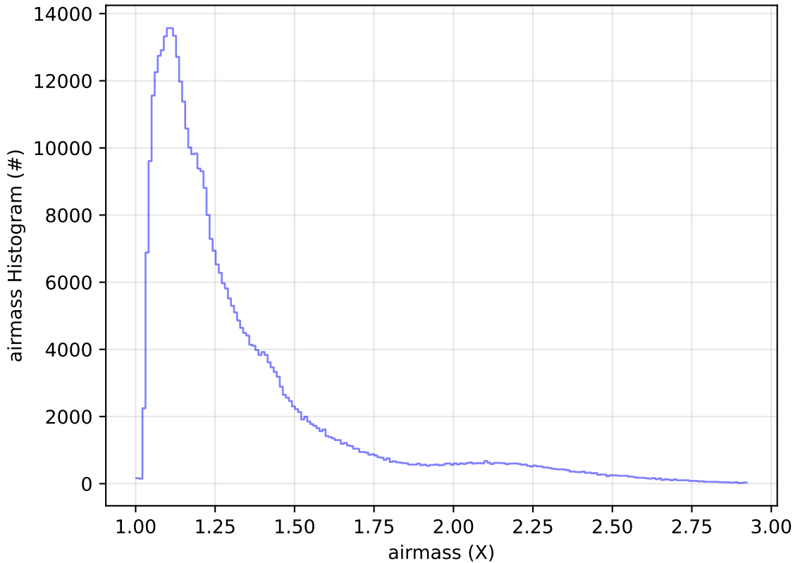
early_ss_template_fpextra2.0_v3.4_10yrs All sky z band: airmass Histogram
