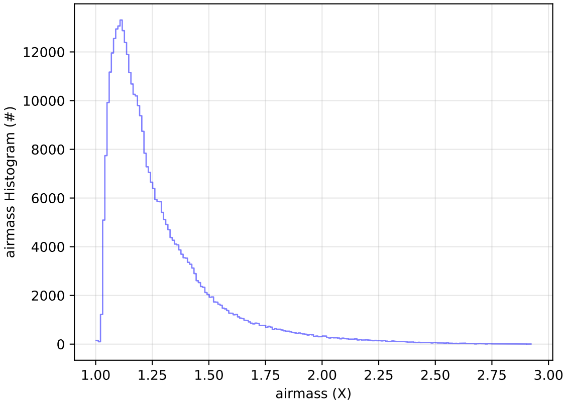
early_ss_template_fpextra2.0_v3.4_10yrs All sky y band: airmass Histogram
