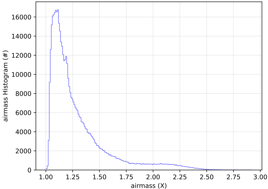
early_ss_template_fpextra2.0_v3.4_10yrs All sky r band: airmass Histogram
