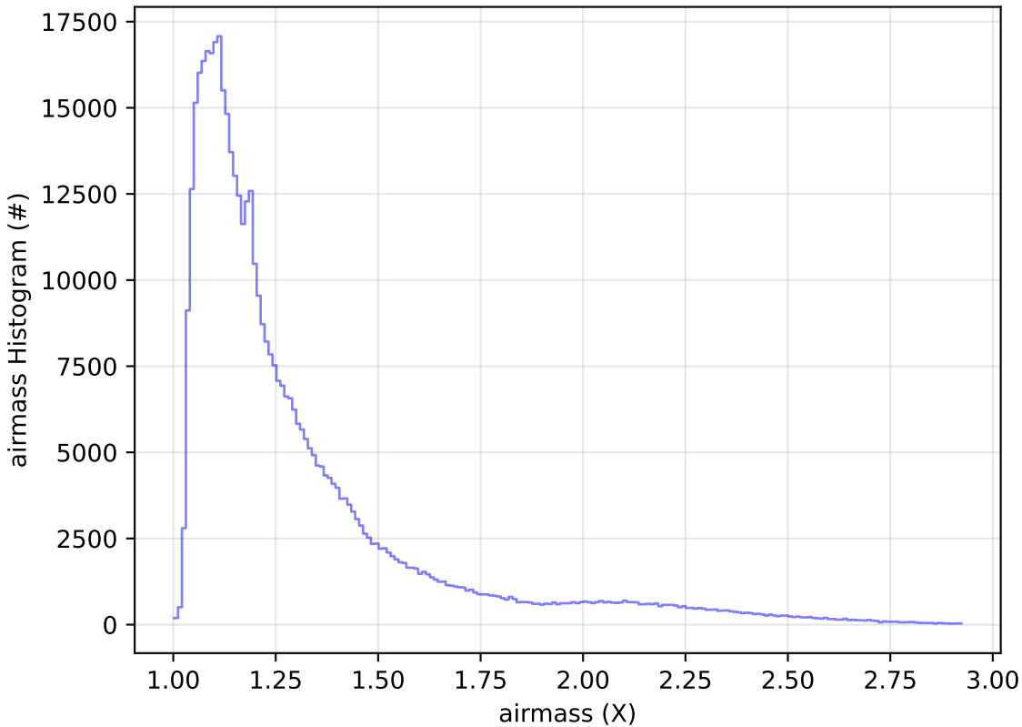
early_ss_template_fpextra2.0_v3.4_10yrs All sky i band: airmass Histogram
