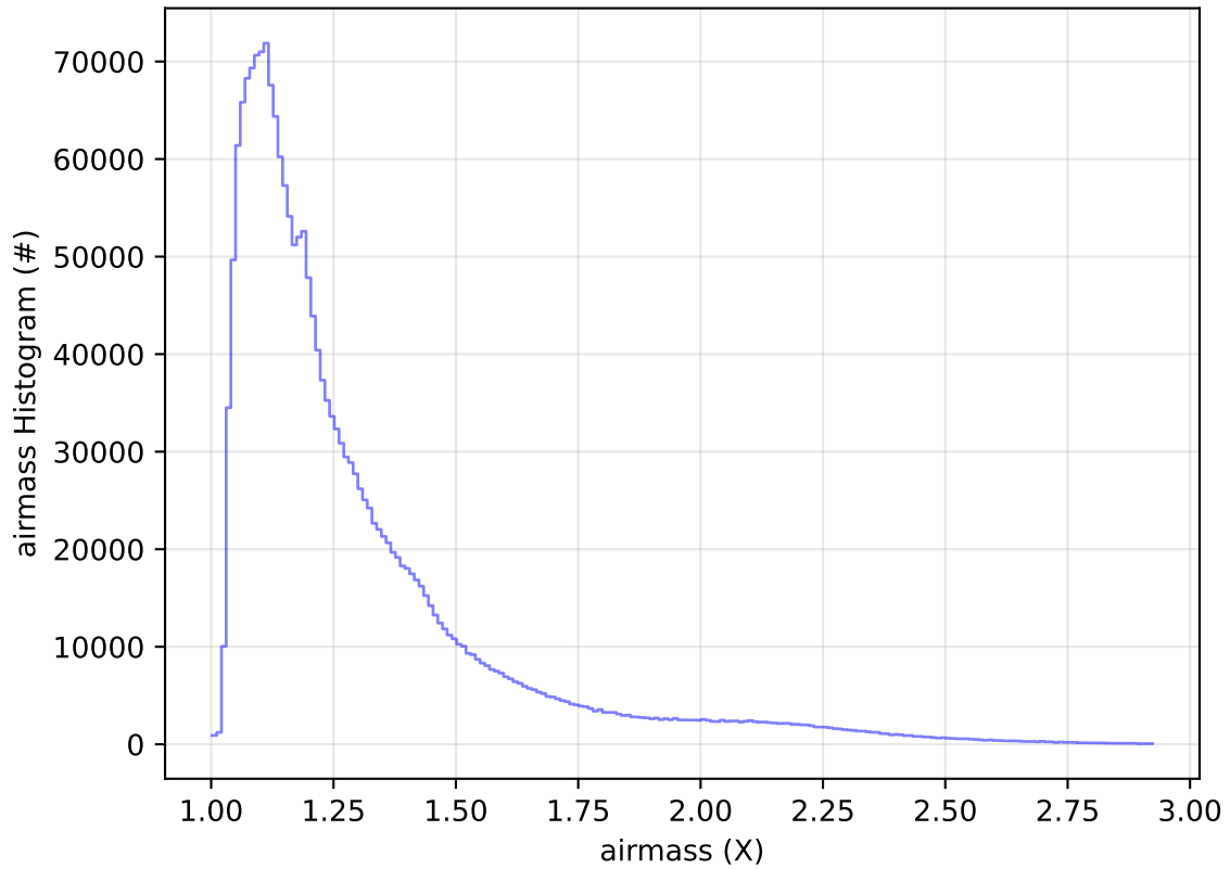
early_ss_template_fpextra2.0_v3.4_10yrs All sky all bands: airmass Histogram
