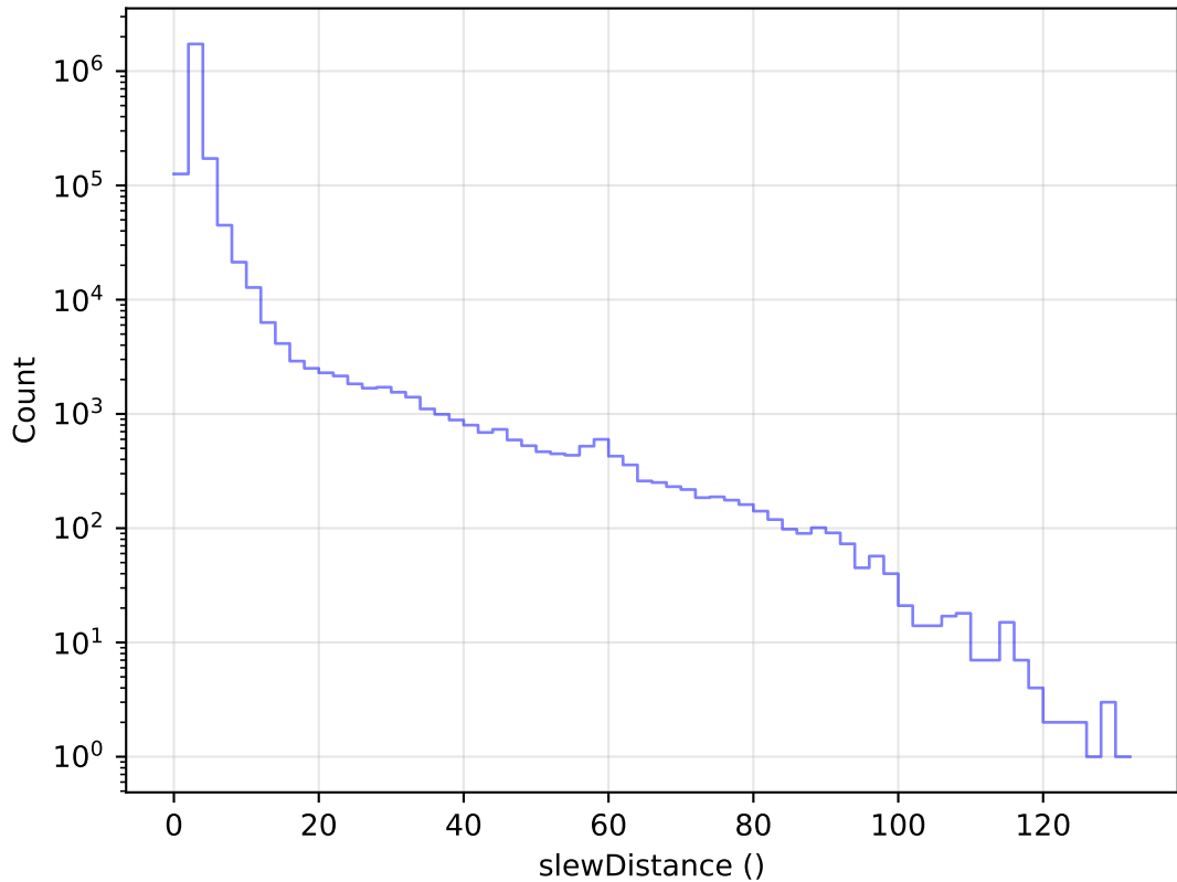
early_ss_template_fpextra2.0_v3.4_10yrs All visits: Slew Distance Histogram
