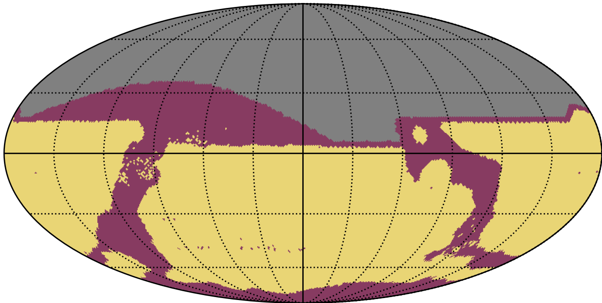
early_ss_template_fpextra2.0_v3.4_10yrs All sky: RapidRevisits
