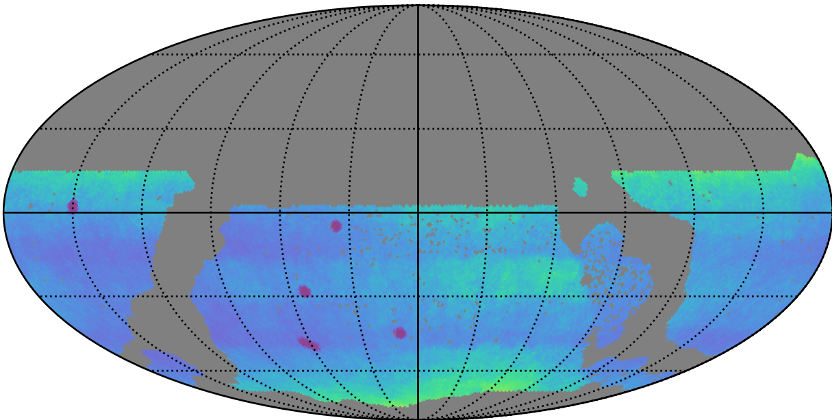
early_ss_template_fpextra2.0_v3.4_10yrs WFD: Proper Motion Uncert @ 24.0
