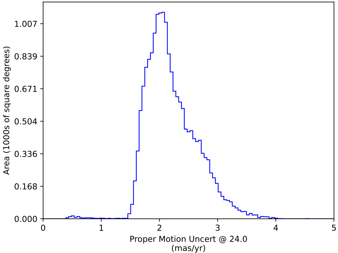
early_ss_template_fpextra2.0_v3.4_10yrs WFD: Proper Motion Uncert @ 24.0
