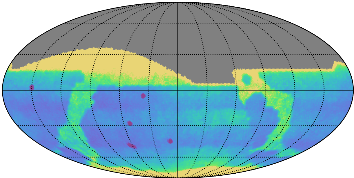
early_ss_template_fpextra2.0_v3.4_10yrs All sky: Proper Motion Uncert @ 24.0
