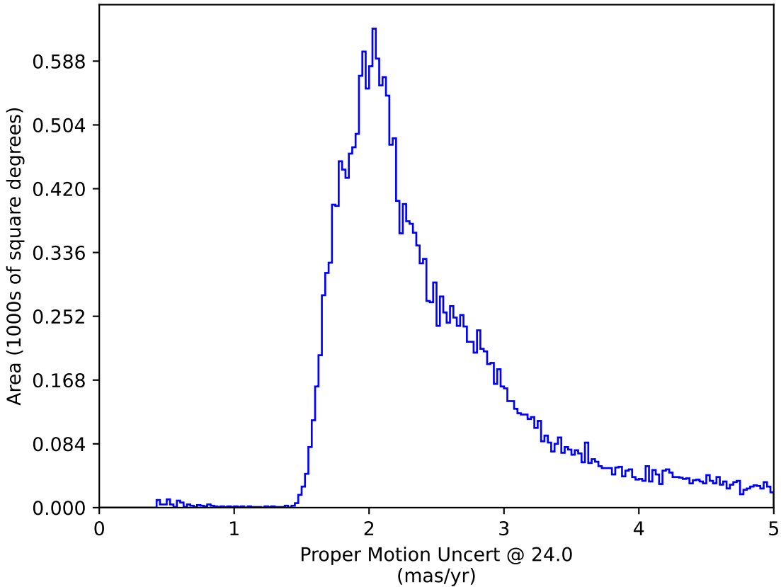
early_ss_template_fpextra2.0_v3.4_10yrs All sky: Proper Motion Uncert @ 24.0
