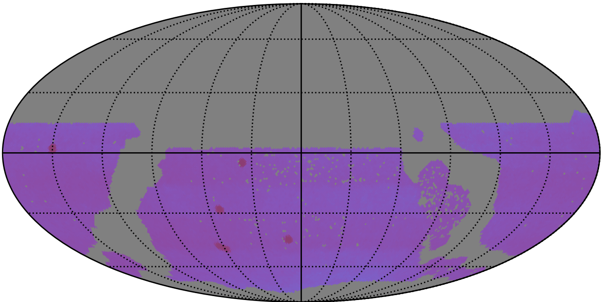
early_ss_template_fpextra2.0_v3.4_10yrs WFD: Proper Motion Uncert @ 20.5
