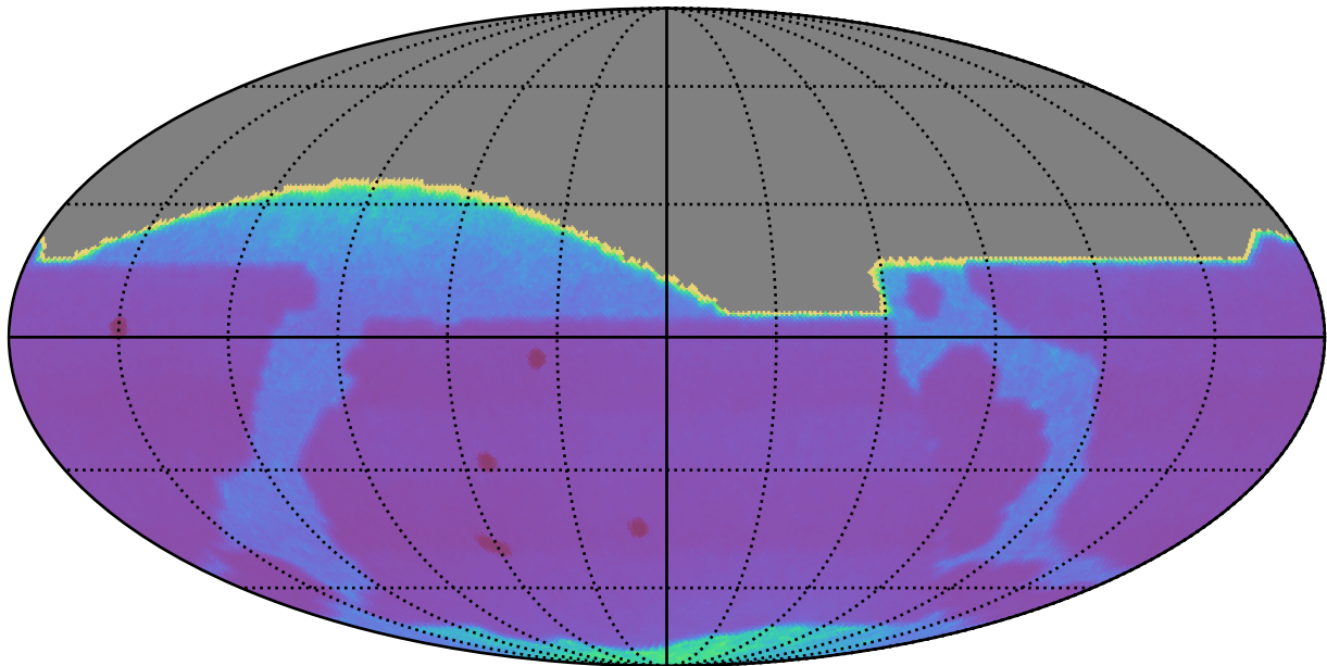
early_ss_template_fpextra2.0_v3.4_10yrs All sky: Proper Motion Uncert @ 20.5
