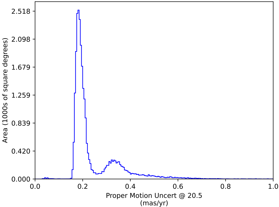
early_ss_template_fpextra2.0_v3.4_10yrs All sky: Proper Motion Uncert @ 20.5
