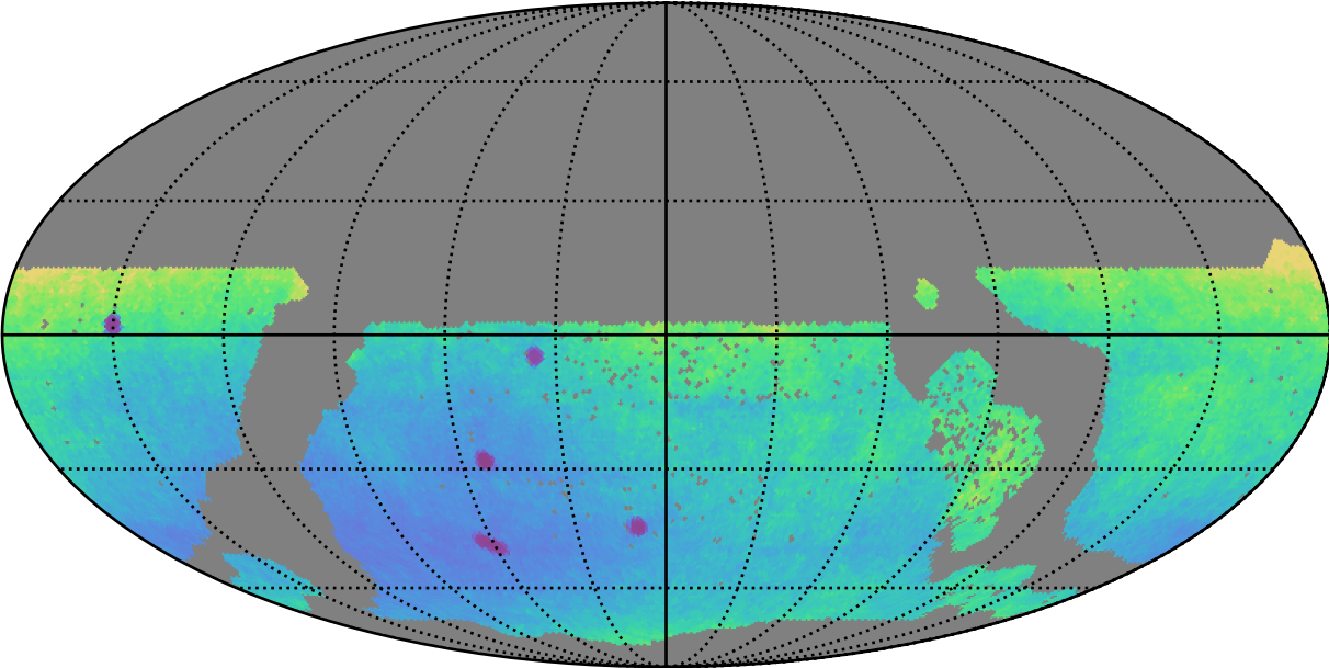
early_ss_template_fpextra2.0_v3.4_10yrs WFD y band only: Parallax Uncert @ 21.3
