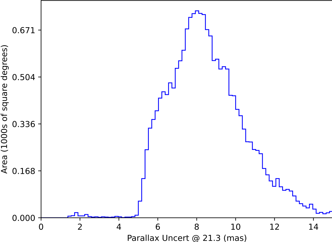
early_ss_template_fpextra2.0_v3.4_10yrs WFD y band only: Parallax Uncert @ 21.3
