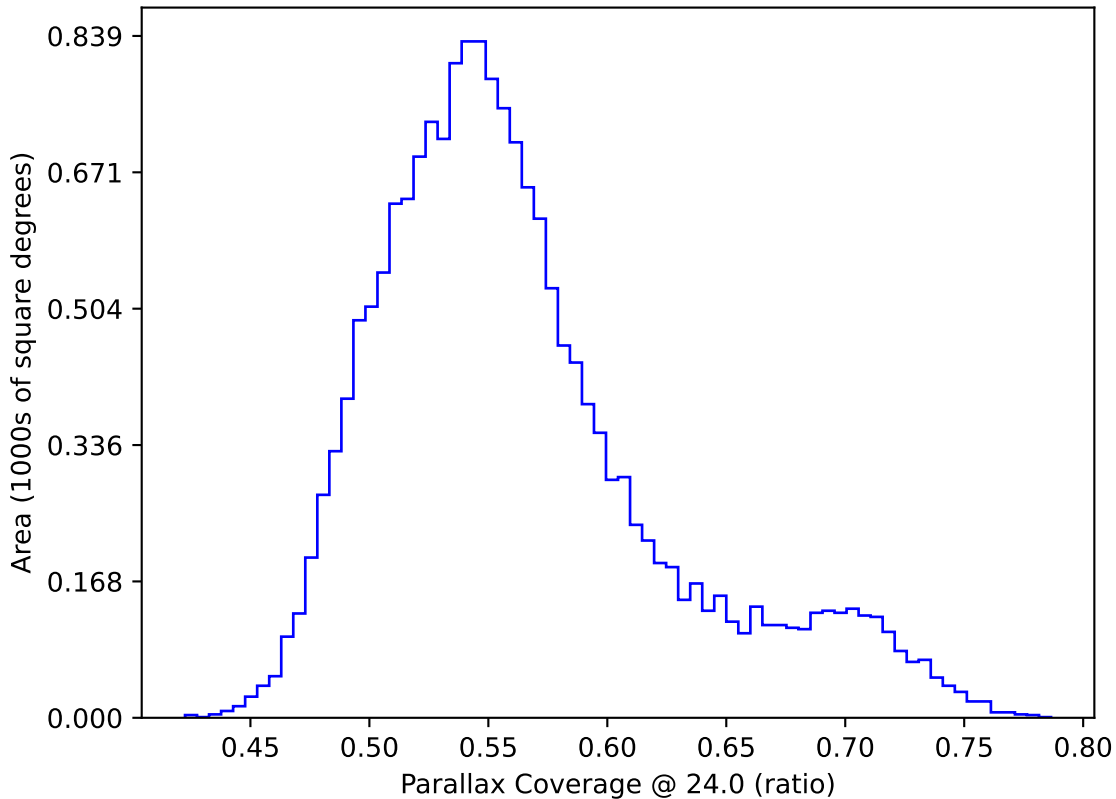
early_ss_template_fpextra2.0_v3.4_10yrs WFD: Parallax Coverage @ 24.0
