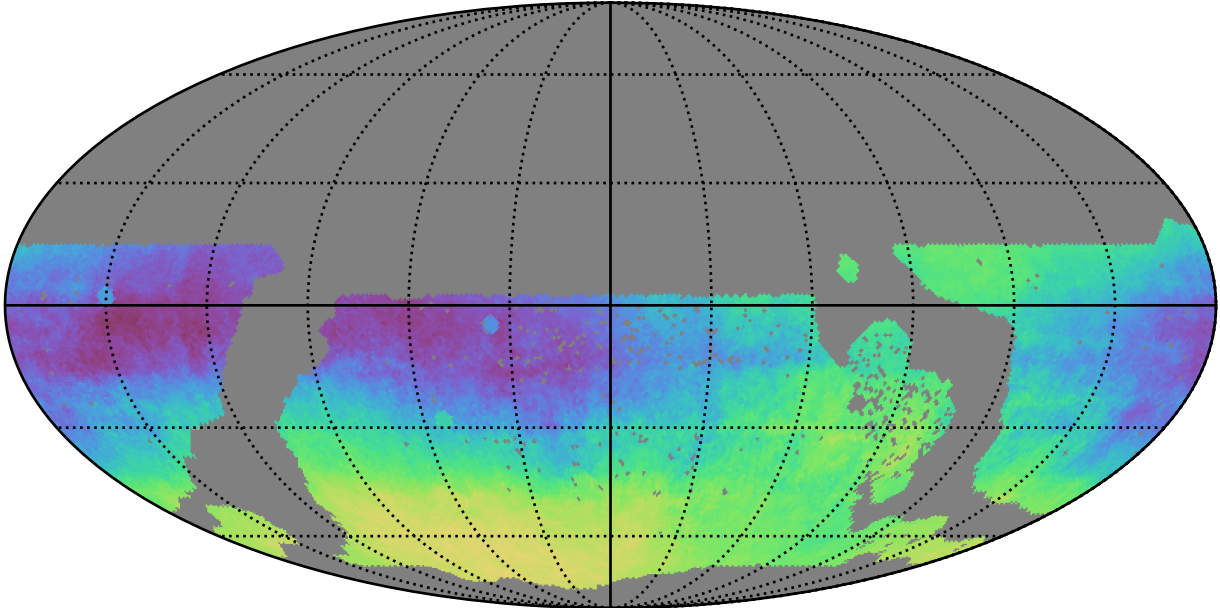
early_ss_template_fpextra2.0_v3.4_10yrs WFD: Parallax-DCR degeneracy @ 24.0
