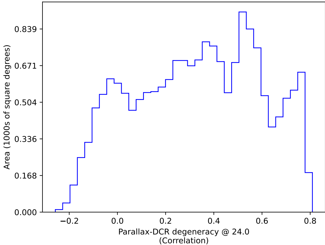
early_ss_template_fpextra2.0_v3.4_10yrs WFD: Parallax-DCR degeneracy @ 24.0
